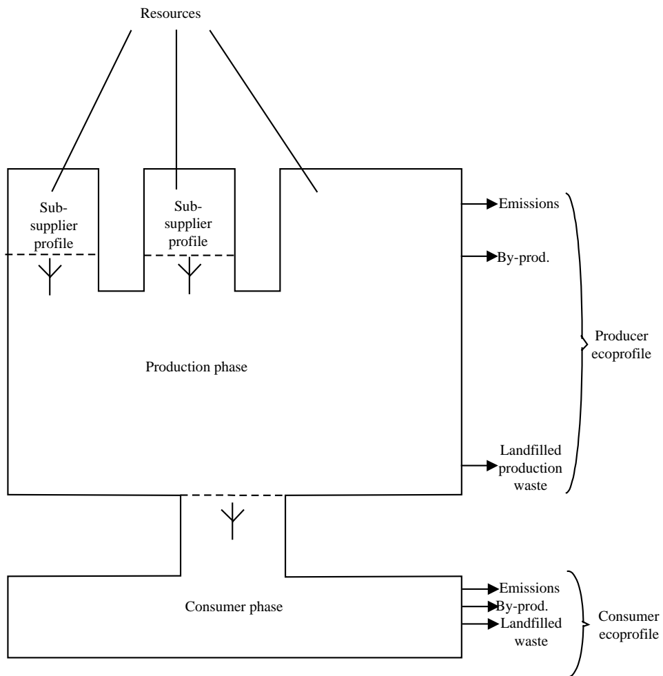
Figure 2. Generalised picture of system boundaries in an ecoprofile analysis. Dashed lines denote boundaries between sub-systems. Arrows symbolise transports of finished goods within the system or, in the case of by-products and waste, away from the system.
