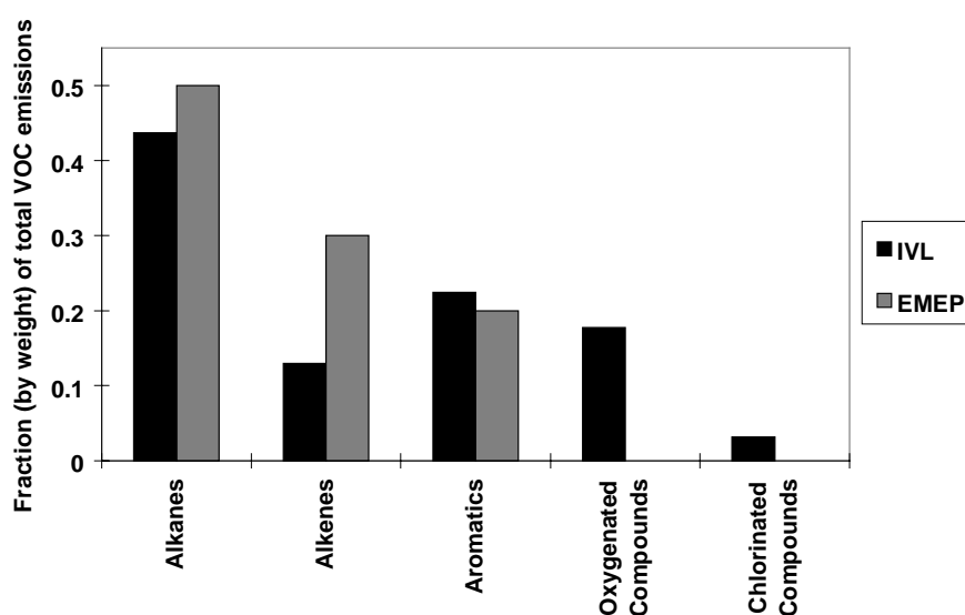
Figure 2.1. The distribution of VOC in different groups of compounds in the IVL and EMEP chemical schemes.
