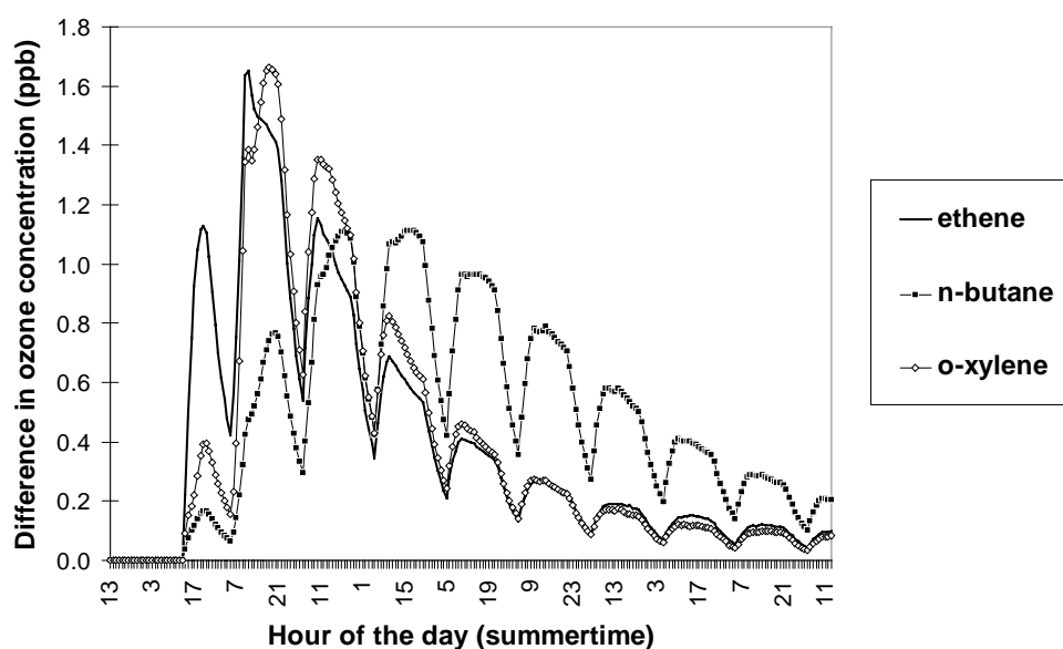
Figure 3.1. The ozone produced from a point source of ethene, n-butane and o-xylene.
