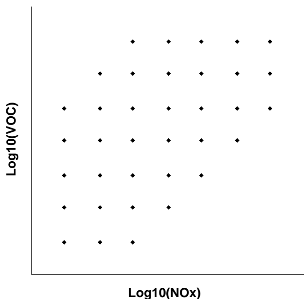
Figure 2.2. The 36 emission scenarios plotted as the logarithm of VOC emission versus the logarithm of NO x emission. Each point refers to a different emission scenario which has been simulated. There are seven different levels of emission rates for both NO x and VOC; 0.03, 0.1, 0.3, 1, 3, 10 and 30 \text{ tonnes}\cdot\text{km}^{-2}\cdot\text{year}^{-1} .
