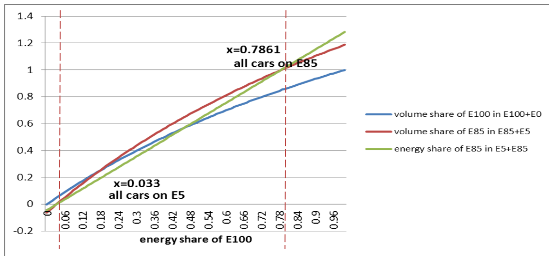
Figure 3. Shares of fuels in the fuel mixture of E5 and E85 as functions of E100 energy share
